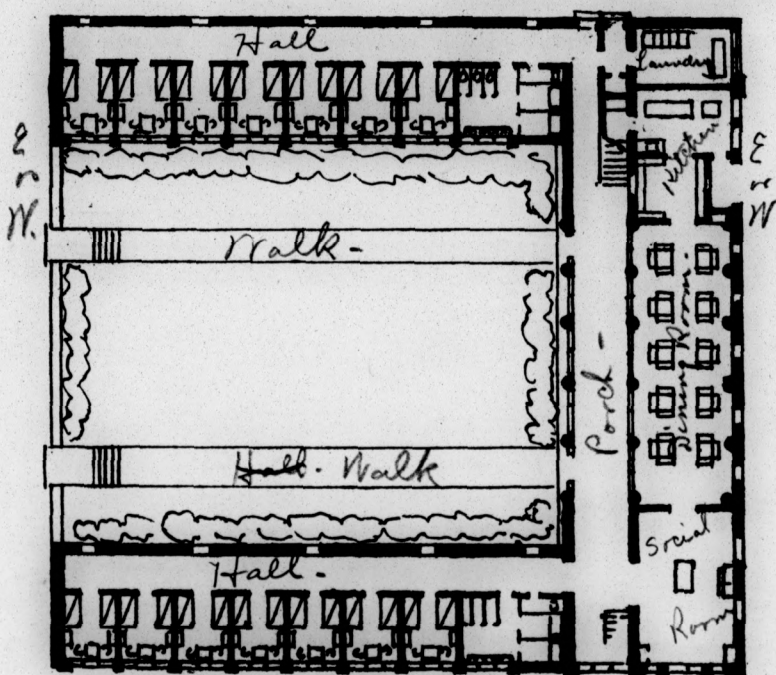
TYPICAL UNIT PLAN. South.
